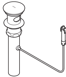
Drain Assembly
